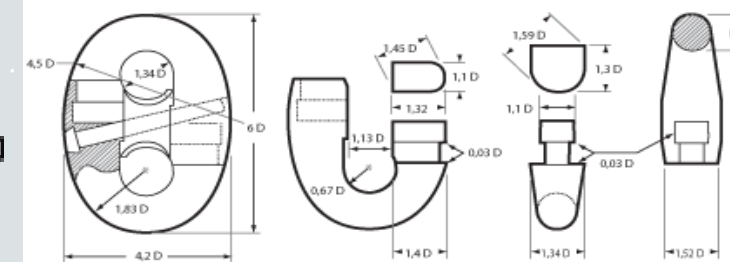
JOINING SHACKLE TYPE KENTER
