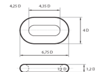
ENLARGED LINK
