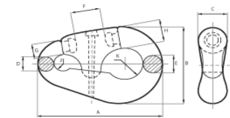
PEAR SHAPED END SHACKLE
