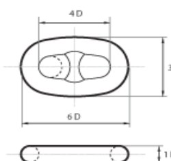
COMMON LINK
