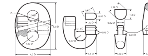
RAMFOR™ SLIM CONNECTORS
