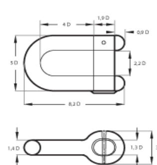
ANCHOR SHACKLE TYPE D
